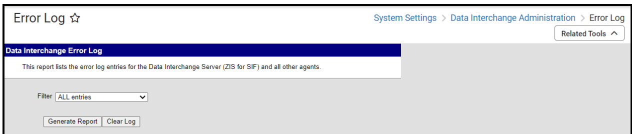
Image 1. Error Log
