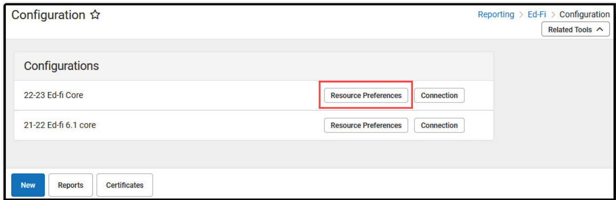
Ed-Fi Configuration
