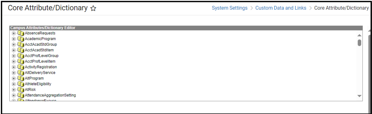
Image 1: Attribute/Dictionary
